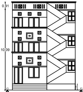
FRONT ELEVATION
