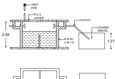
SEPTIC TANK & D-TRENCH DETAILS [ NOT TO SCALE ]
