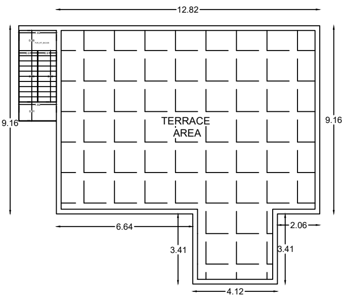
PRO.TERRACE FLOOR PLAN
