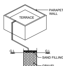
COLLECTION SUMP FOR HARVESTING FOR TERRACE
