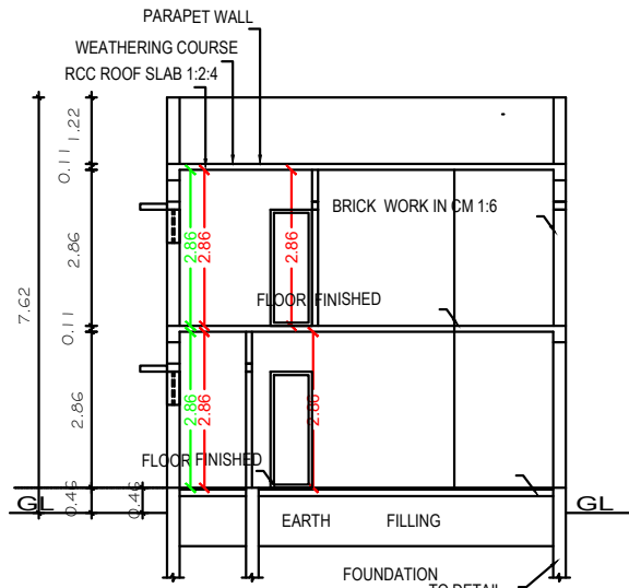
SECTION "X-Y"
