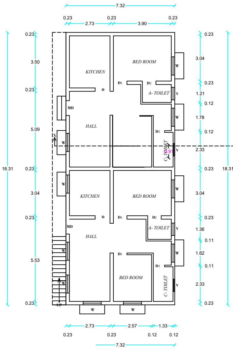
ID FLOOR PLAN
