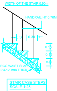
STAIR CASE STEPS SCALE 1:25
