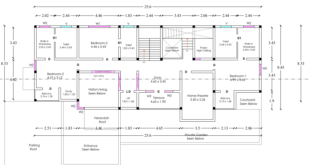
PRO-FIRST FLOOR PLAN BLOCK-1
