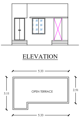
PRO-TERRACE PLAN BLOCK-2
