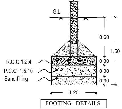
FOOTING DETAILS
