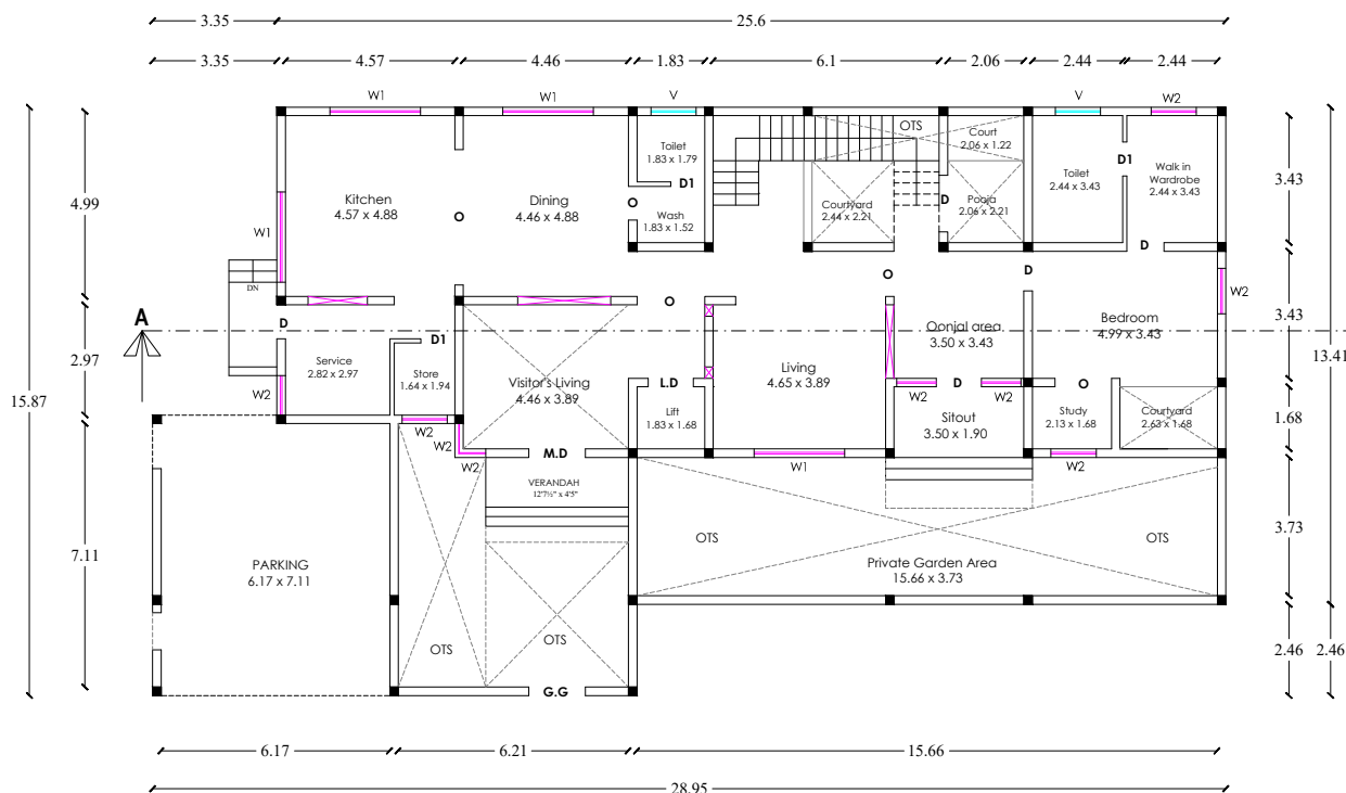
PRO-GROUND FLOOR PLAN BLOCK-1
