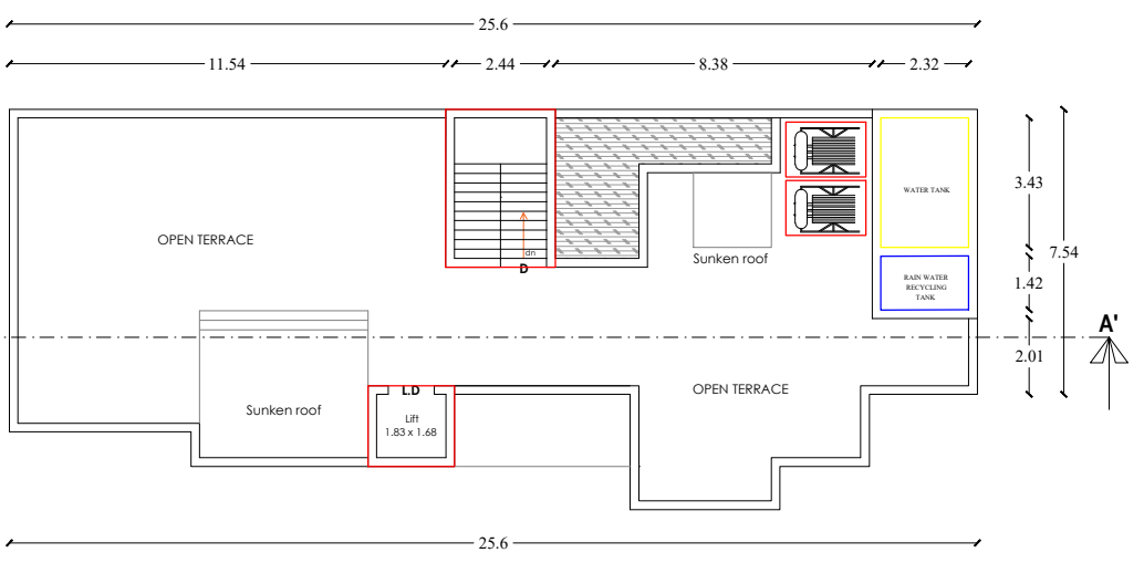
PRO-TERRACE PLAN BLOCK-1
