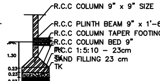
SECTION
