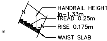
STAIRCASE DETAILS
