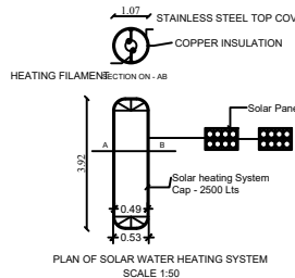
PLAN OF SOLAR WATER HEATING SYSTEM SCALE 1:50
