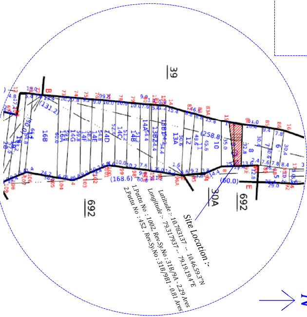
KEY PLAN - SCALE 1:200
