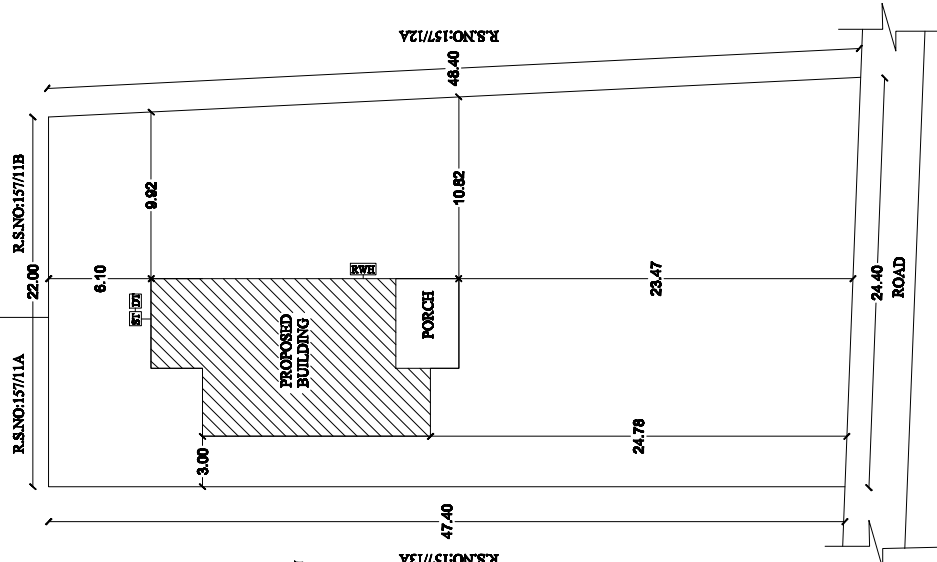
SITE PLAN SCALE 1:200
