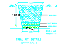
TRIAL PIT DETAIL NOT TO SCALE
