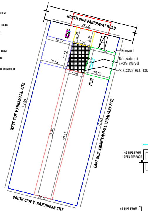
SITE PLAN
