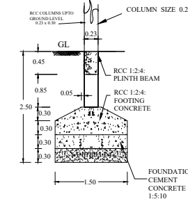
FOUNDATION DETAILS Scale 1:50
