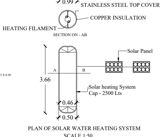
PLAN OF SOLAR WATER HEATING SYSTEM SCALE 1:50
