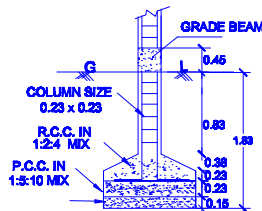
COLUMN DETAILS
