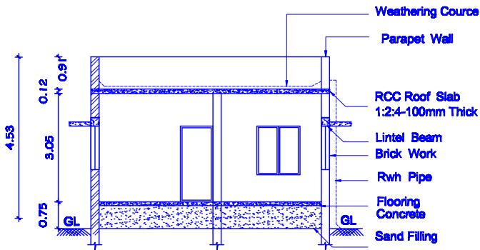
SECTION -XY
