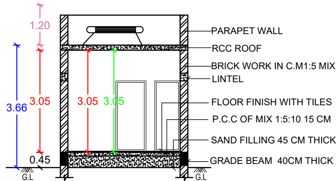
SECTION-AA1
