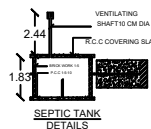
SEPTIC TANK DETAILS
