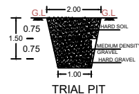
TRIAL PIT
