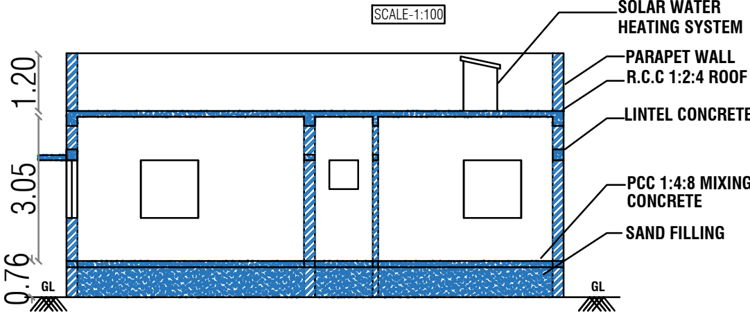
SECTION NO - "AB"
