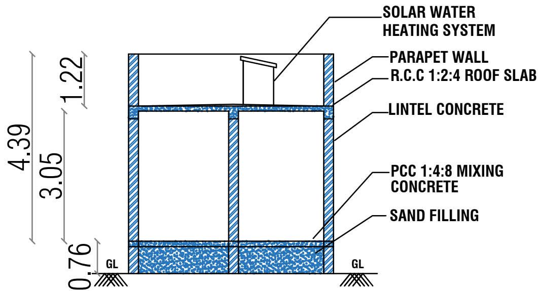
SECTION NO -"AB"
