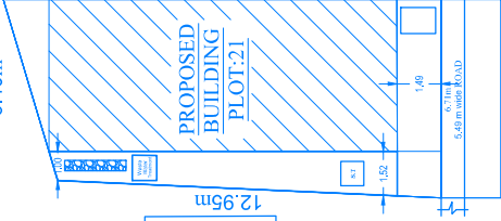
SITE PLAN SCALE:1:100
