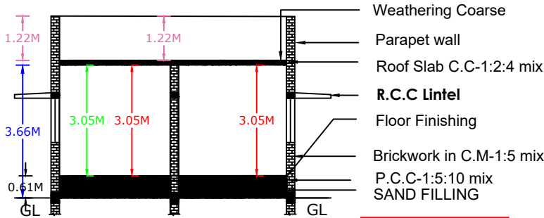
SECTION ON XX
