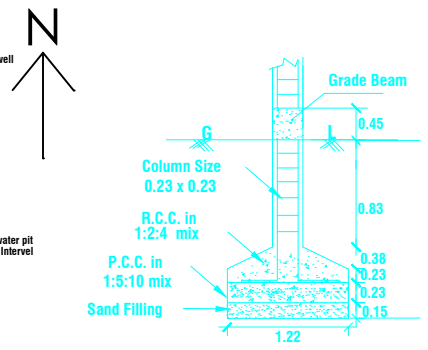
COLUMN DETAILS
