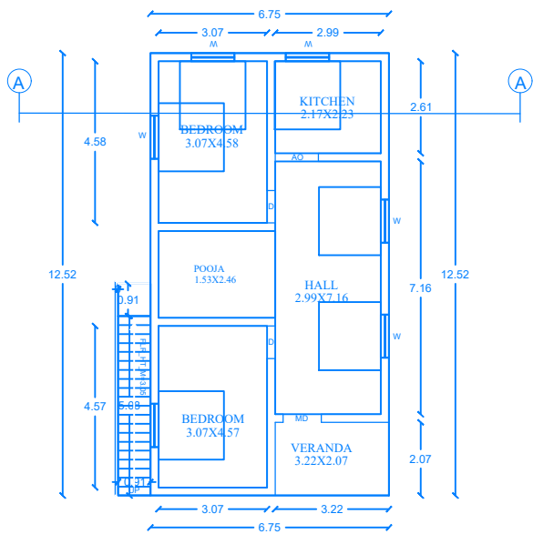
D. GROUND FLOOR PLAN
