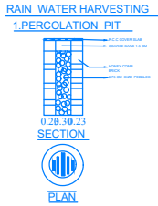
RAIN WATER HARVESTING 1. PERCOLATION PIT
