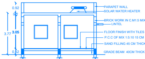
SECTION ON A-A1
