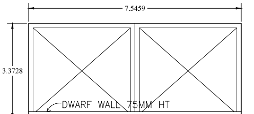
MAIN GATE ELEVATION
