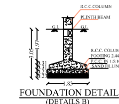
FOUNDATION DETAIL (DETAILS B)
