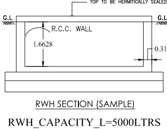
RW SECTION (SAMPLE)
