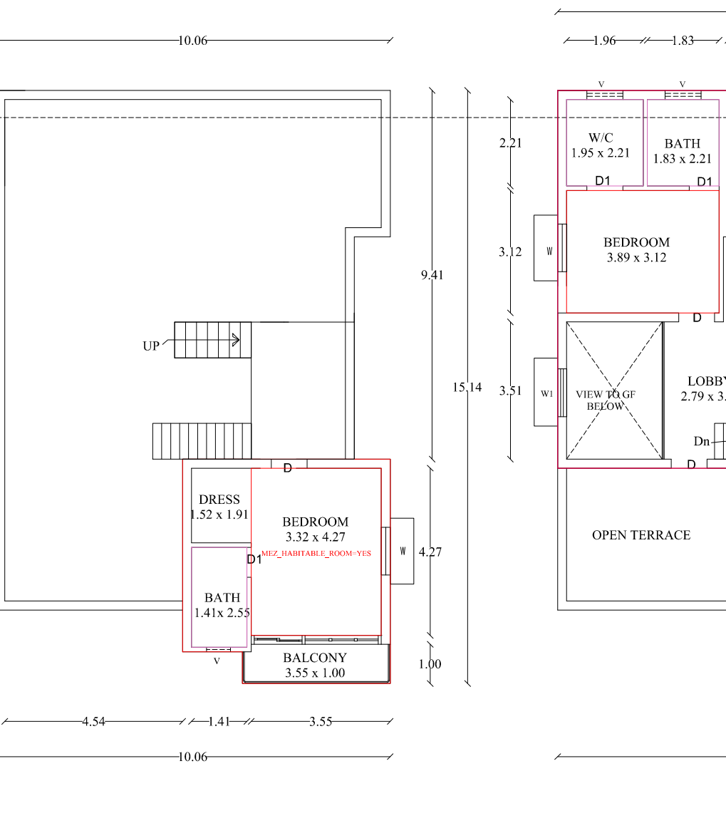
PRO - FIRST MEZZANINE FLOOR PLAN
