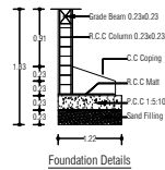
Foundation Details
