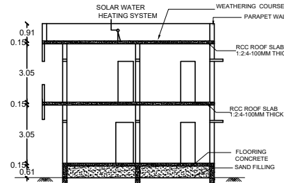
SECTION NP
