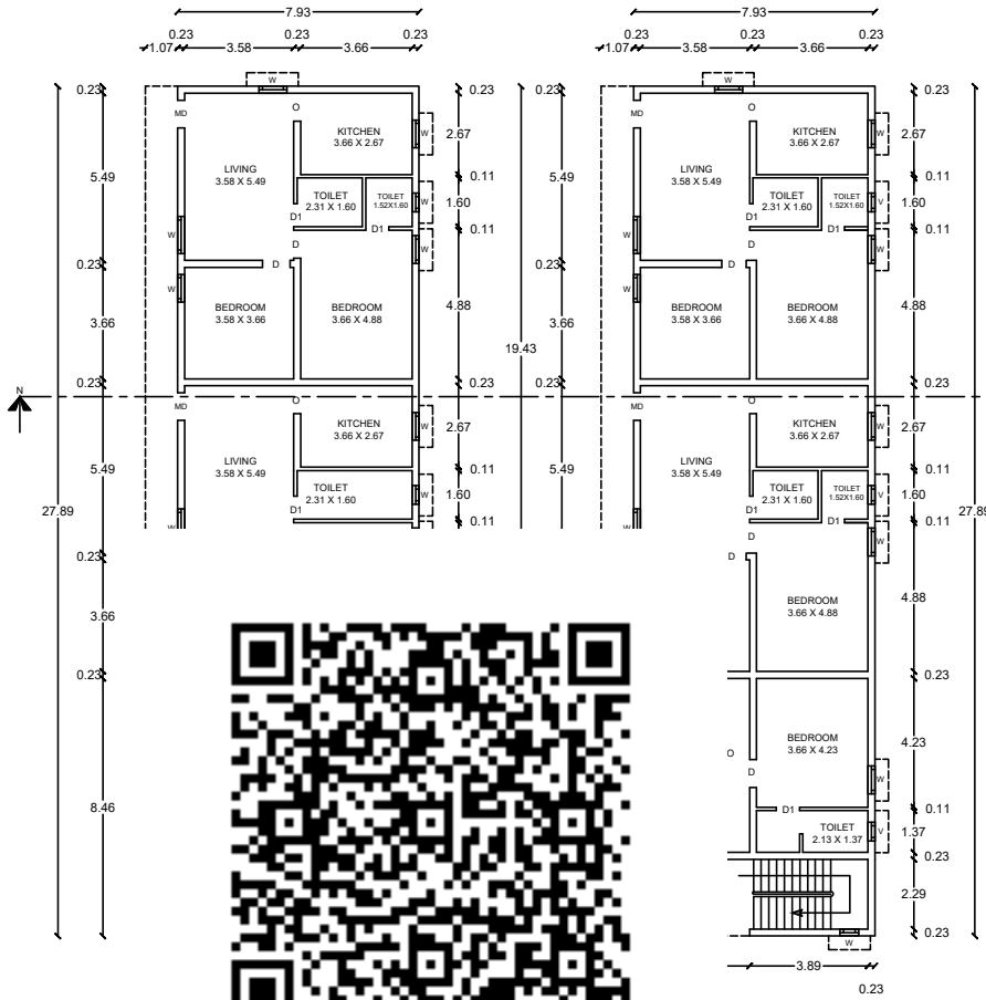
FLOOR PLAN
