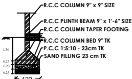
SECTION
