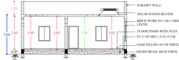
SECTION- AA1
