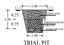
TRIAL PIT
