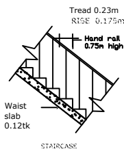
STAIRCASE
