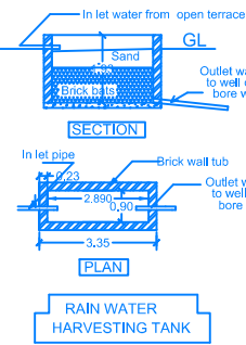
RWH_CAPACITY_L = 2000LTRS
