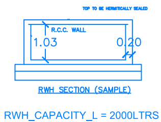
RWH_CAPACITY_L = 2000LTRS
