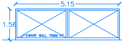
MAIN GATE
