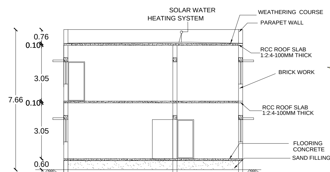
SECTION ON BR
