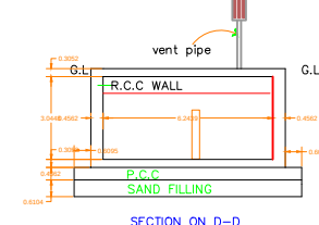
SECTION ON D-D
