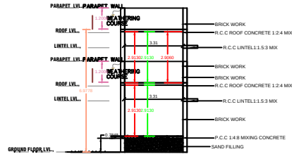
CROSS SECTION
