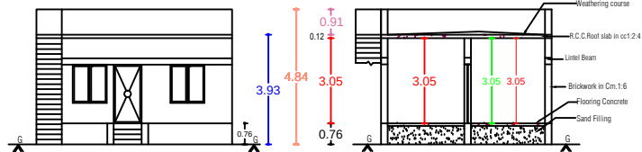
FRONT ELEVATION
