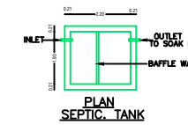
PLAN SEPTIC. TANK
