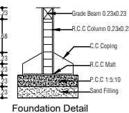
Foundation Detail
