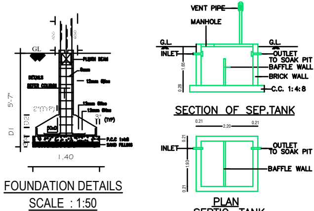
PLAN SEPTIC. TANK
