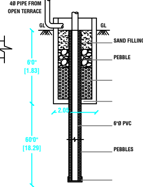
Section of Rain water Harvesting (from open terraced)
