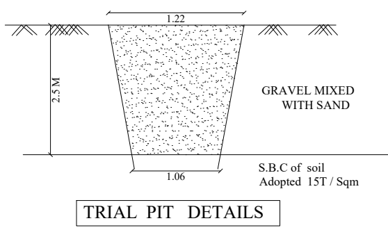
TRIAL PIT DETAILS
