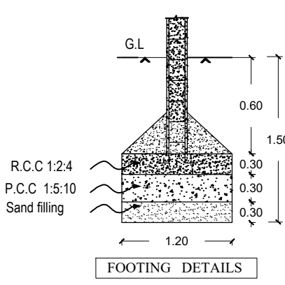
FOOTING DETAILS
