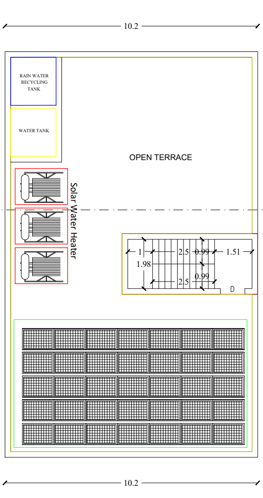
TERRACE PLAN
