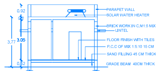
SECTION ON A-A1
