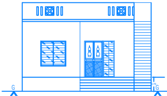
FRONT ELEVATION
