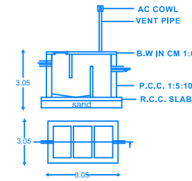
Septic tank detail
