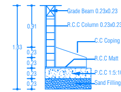
Foundation Details
