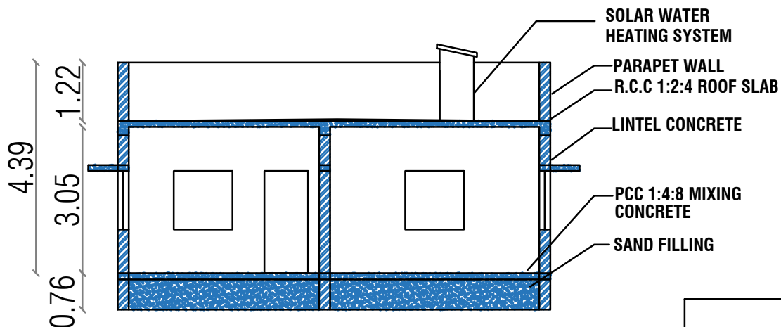
SECTION NO -"AB"
