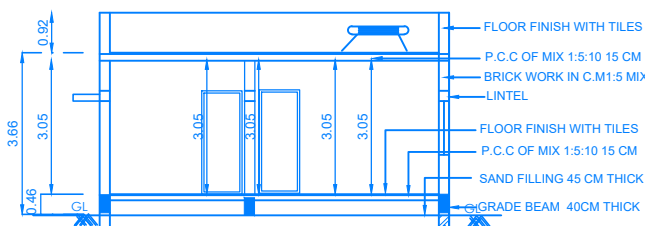
SECTION ON A-A1
