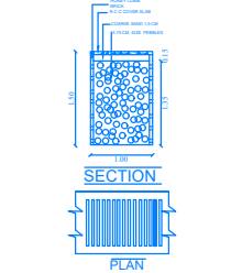
RAIN WATER HARVESTING PERCOLATION BED
