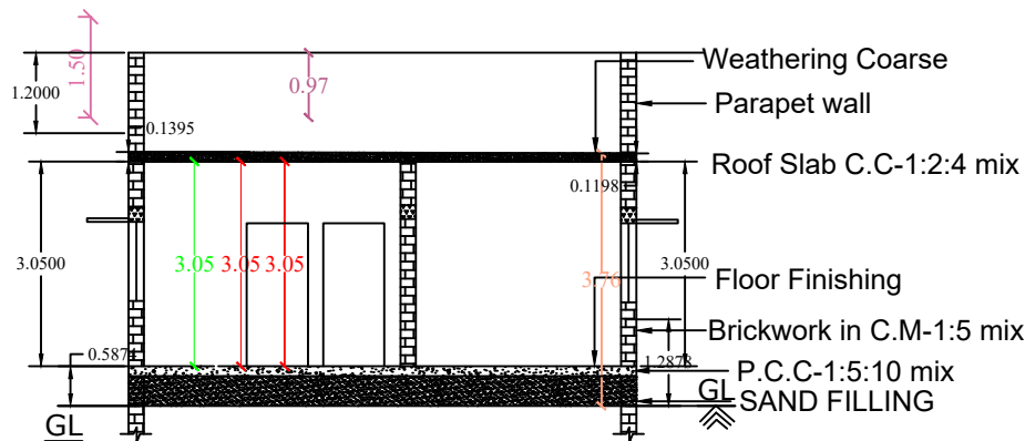
CROSS SECTION ON XX
