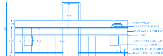
SECTION ON A-A1
