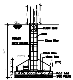
FOUNDATION DETAILS
