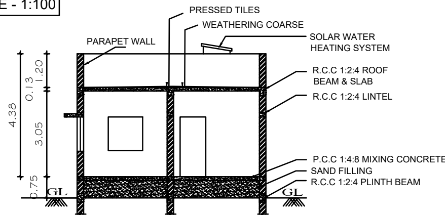
SECTION "A-B"
