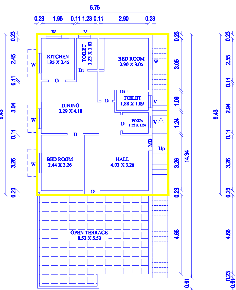
EXTG - FIRST FLOOR PLAN
