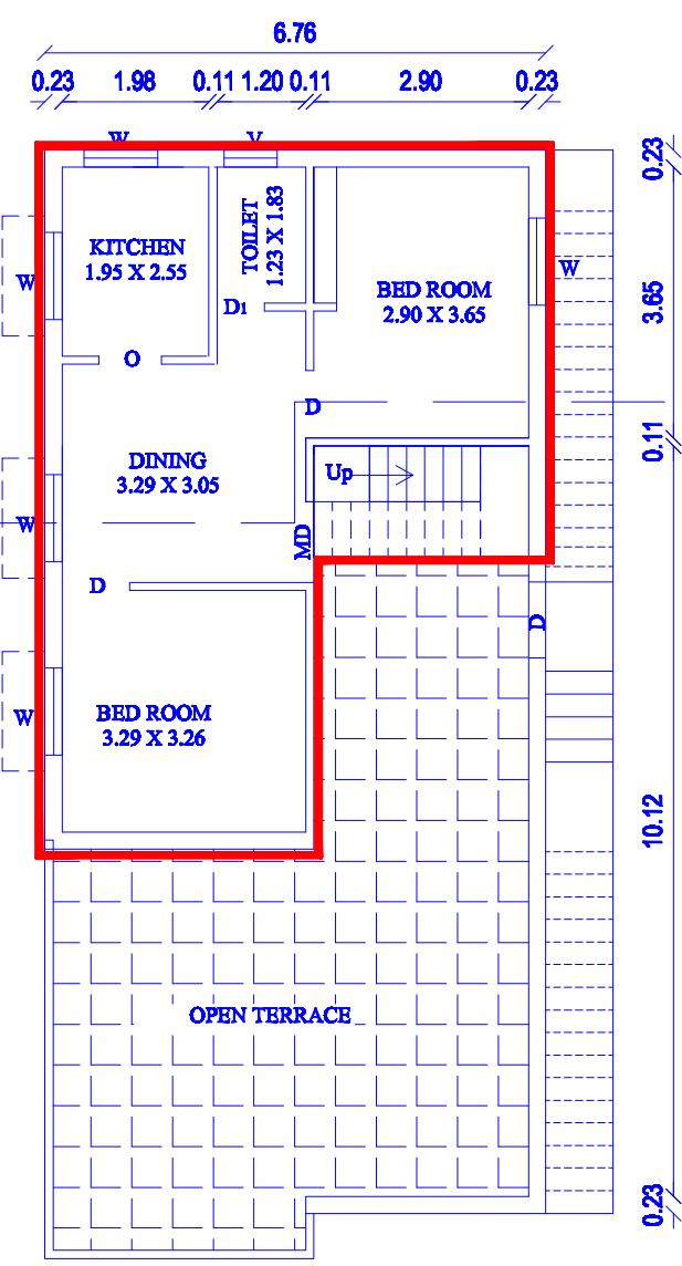
PRO - SECOND FLOOR PLAN
