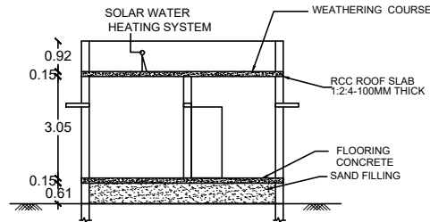
SECTION NP
