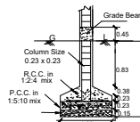
COLUMN DETAILS NOT TO SCALE
