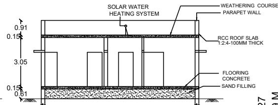
SECTION NP
