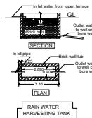
RAIN WATER HARVESTING TANK
