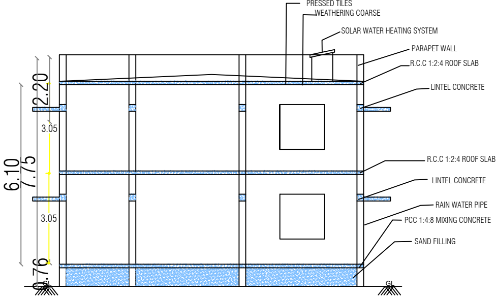
SECTION NO -"AA"
