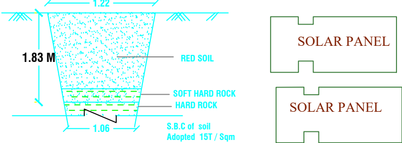
TRIAL PIT DETAILS NOT TO SCALE
