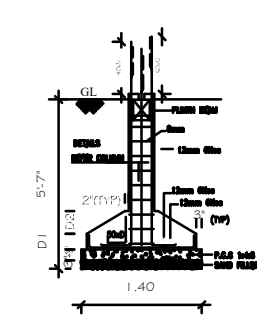
FOUNDATION DETAILS SCALE : 1:50
