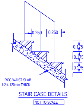
STAIR CASE DETAILS NOT TO SCALE
