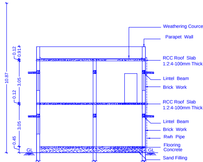
SECTION X-Y
