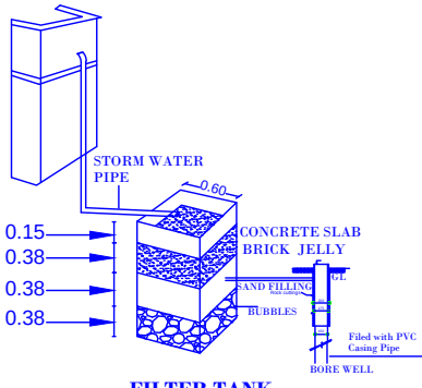
FILTER TANK RAIN WATER HARVESTING
