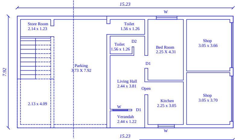
Floor Plan
