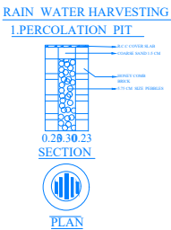
RAIN WATER HARVESTING I PERCOLATION PIT
