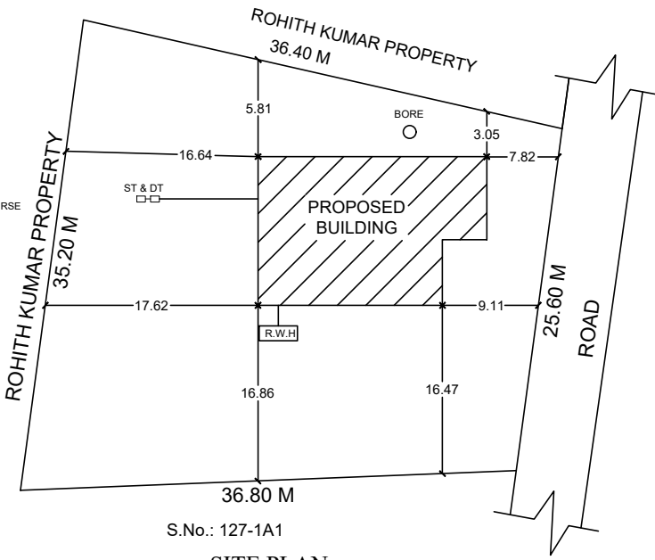
SITE PLAN
