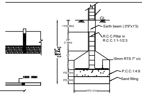
FOUNDATION DETAILS
