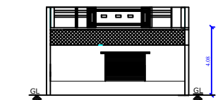
FRONT ELEVATION
