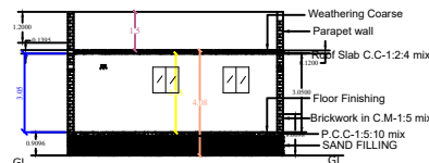
SECTION ON-AB
