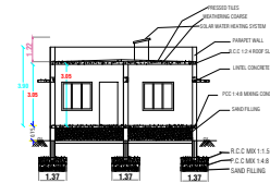
SECTION NO - "AA"
